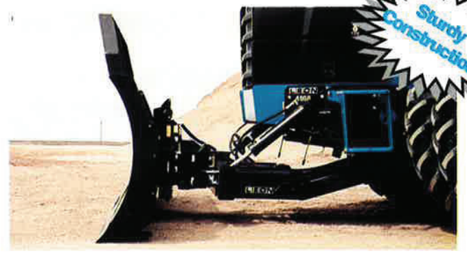
Sturdy Construction and Mounting is featured to insure these units stand up in the toughest of conditions. Push pressure is transmitted from the rear of the front tractor section & is designed to place minimum stress on the tractor framework. All hydraulics included.
